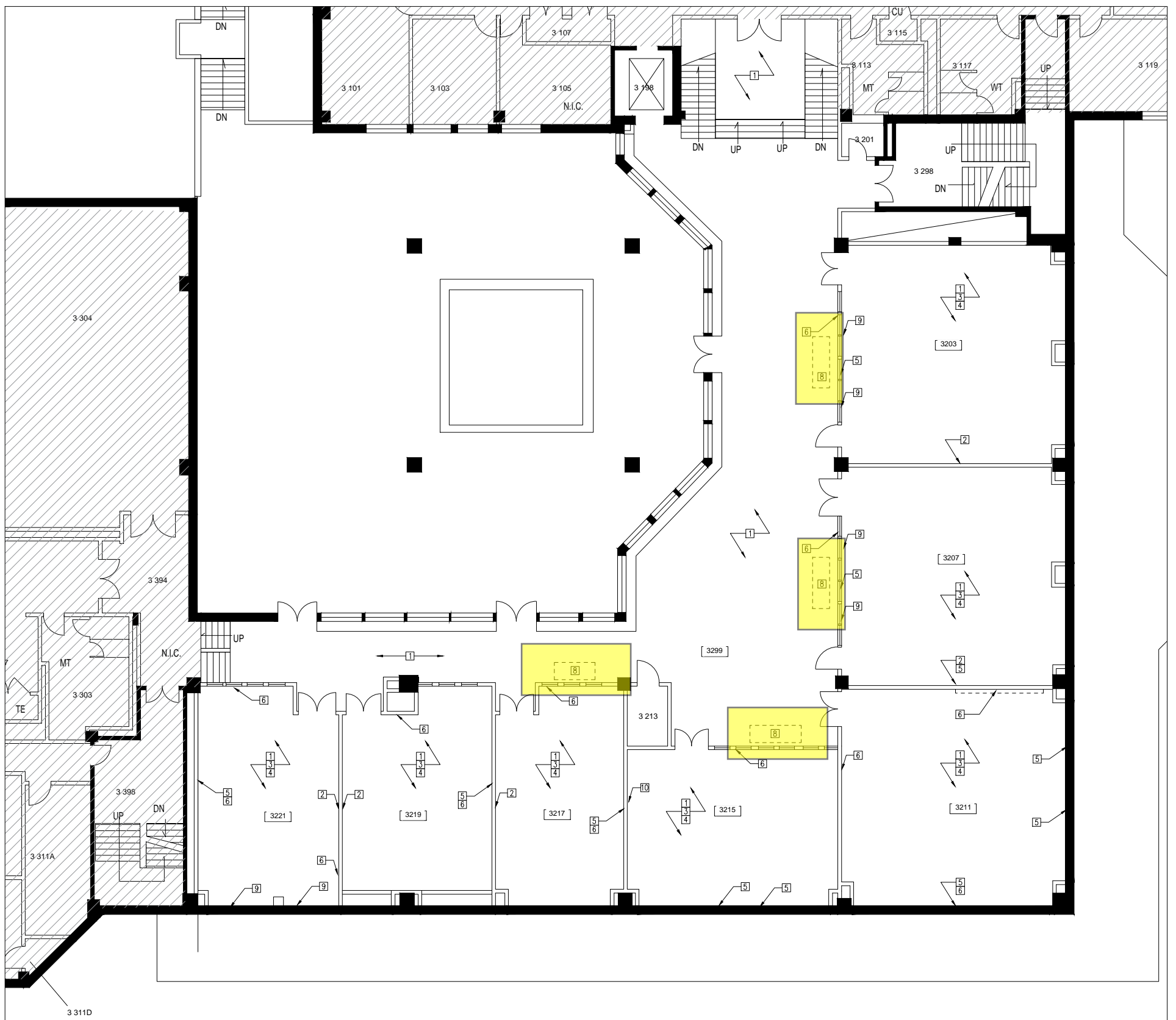
1 THIRD FLOOR PLAN: DEMOLITION SCALE: 1/8"=1'-0"
